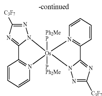
Os(hptz) 2 (PPh 2 Me) 2
