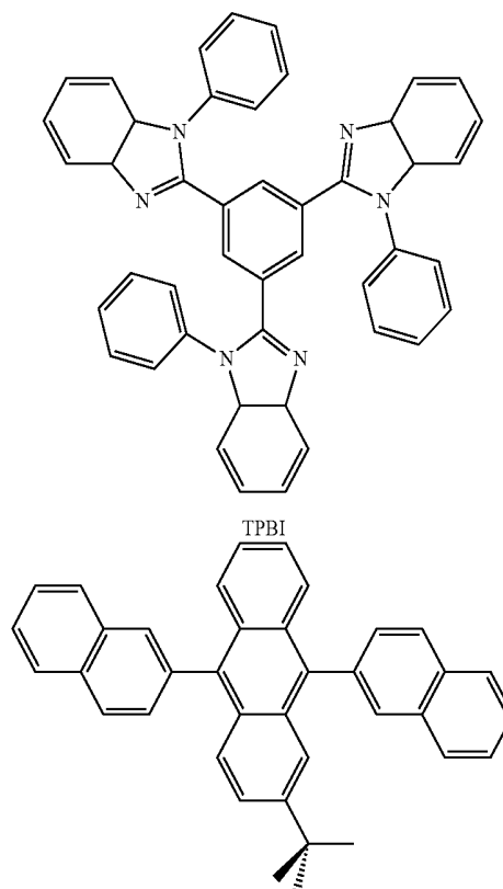
TBADN
