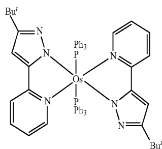
Os(bppz) 2 (PPh 3 ) 2
